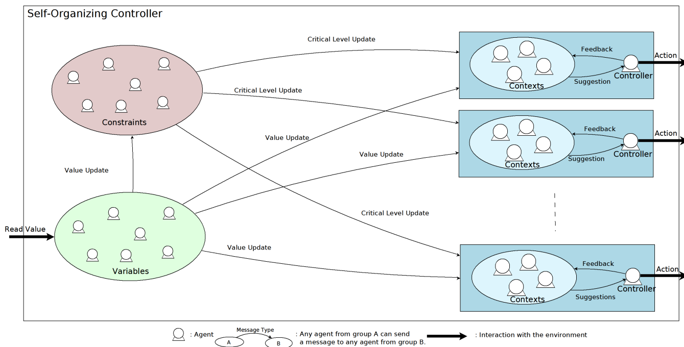
Figure 1: SOC Topology
